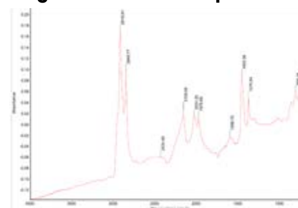
Figure 3: 0.2_5.0 (T) FTIR
