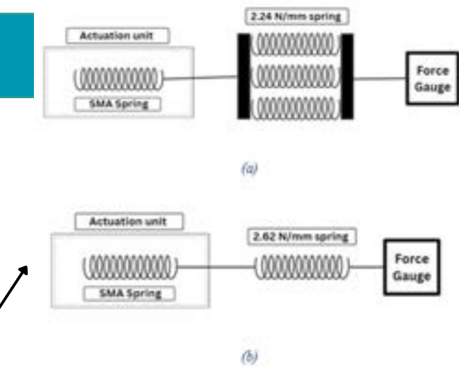
Schematic diagram of Biomechanical modelling. (a) a mimic of cheek muscles (b) a mimic of forehead muscle
