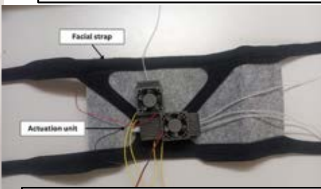
Prototype of the SMA-based facial rehabilitation device
