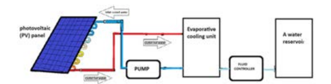
Figure 1 Design of the proposed cooling system model for PV Panels
