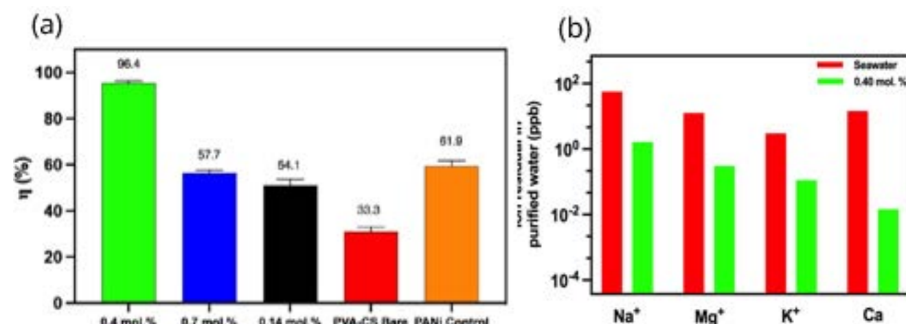
Fig. 4: (a) SVG efficiency of PVA-CS/PANi hydrogel as a function of different APS concentrations and (b) Primary ions concentration of seawater from Pantai Tapang before and after SVG.
