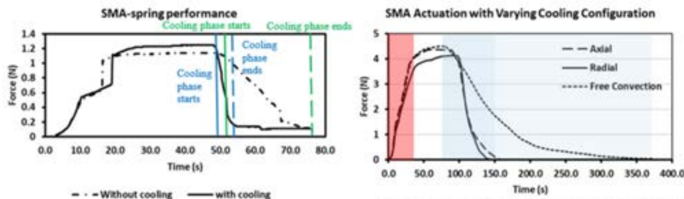
SMA spring performance with cooling (solid) and without cooling (dashed) mechanism
